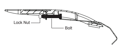
Figure C.3 - Side View
